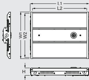
KT-HBLED95PS-1G-8CSD-VDIM /G3
