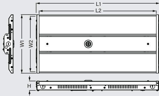
KT-HBLED95PS-1G-8CSD-VDIM /G3
