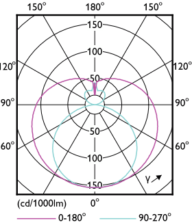
Light Distribution Diagram - 13.4T8/CNG/48-850/MX18/G 25/1
