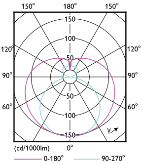
Light Distribution Diagram - 13.4T8/CNG/48-835/MX17/G 25/1
