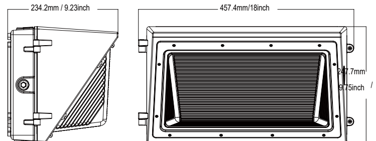
150W Model
