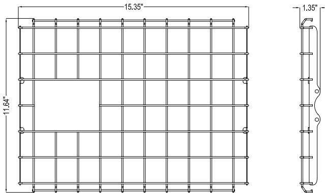
Wire Guard for CLHB-1 & CLHB-2 (130W/165W)
