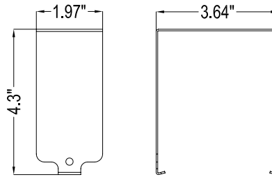
Surface Mount
