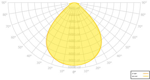
Candela Polar Plot
