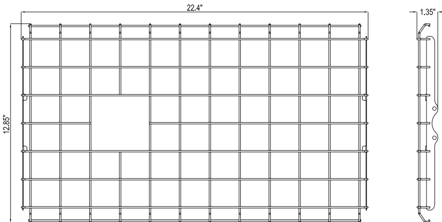
Wire Guard for CLHB-4 (320W)
