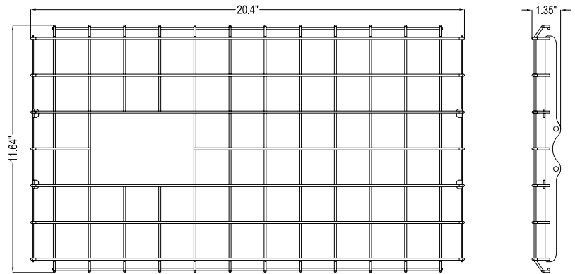
Wire Guard for CLHB-3 (220W)
