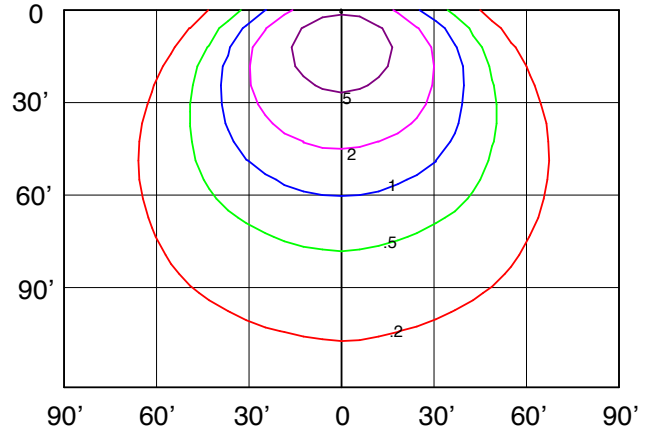
MSF150 Wide 30' Setback 45° Tilt
