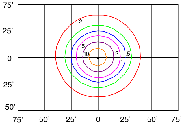
MSF80 Narrow 25' setback
