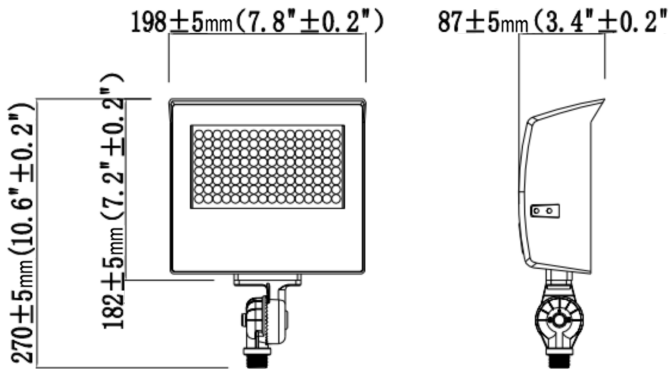
Threaded Knuckle
