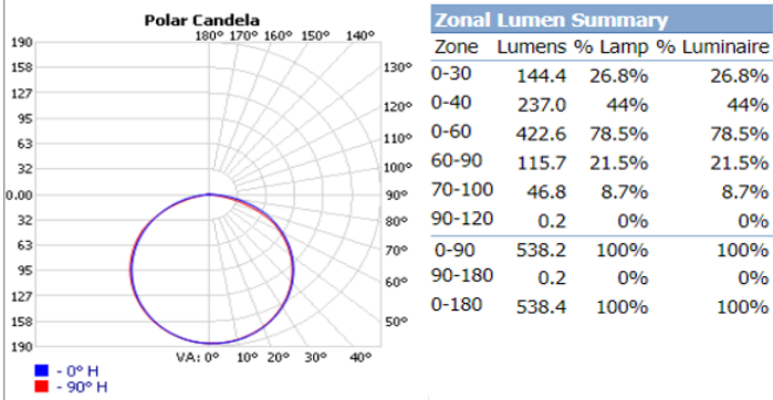
FSDLS3FR8/CCT/LED Settings: 8W at 2700K
